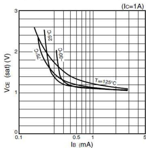
V_{CE(sat)} - I_B Characteristics (Typical)
