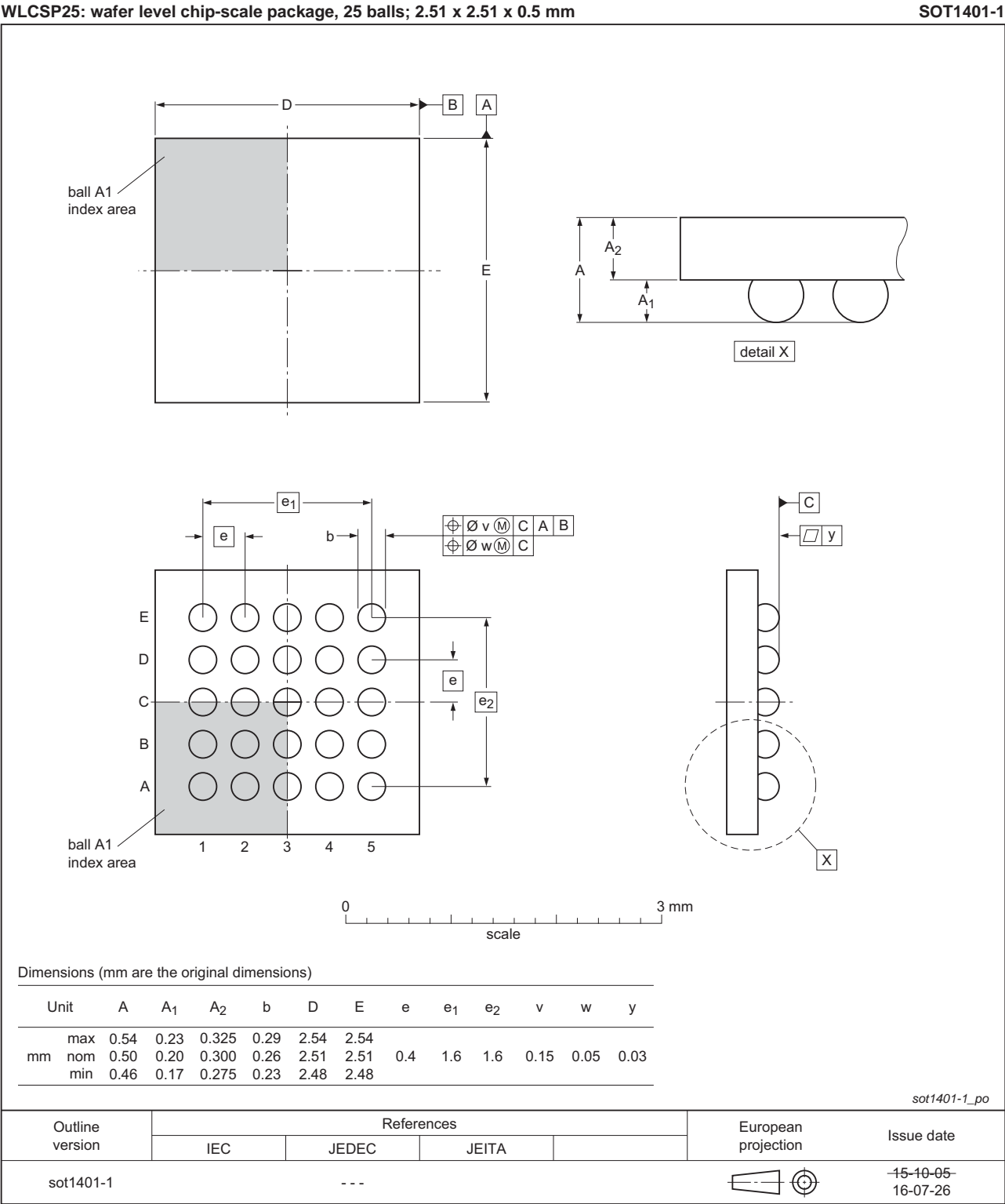
Fig 20. WLCSP25 package outline
