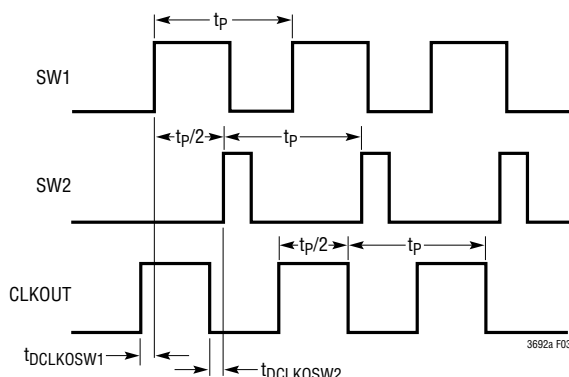
Figure 3. Timing Diagram R_{T/SYNC} = 28.0k , t_p = 1\mu s , V_{D1V} = 0V
