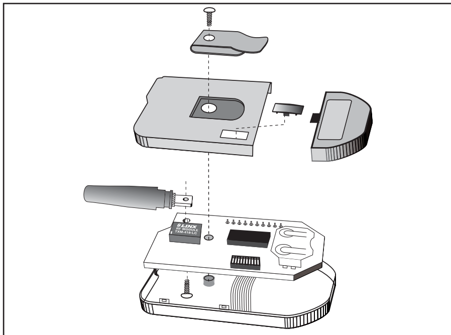
Figure 5: CMD-HHLR-*** Assembly
