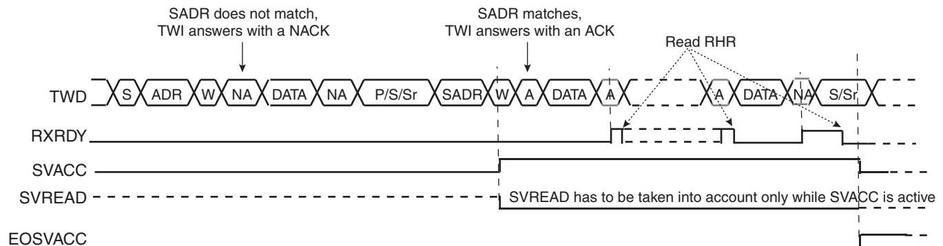
Figure 33-26. Write Access Ordered by a Master
