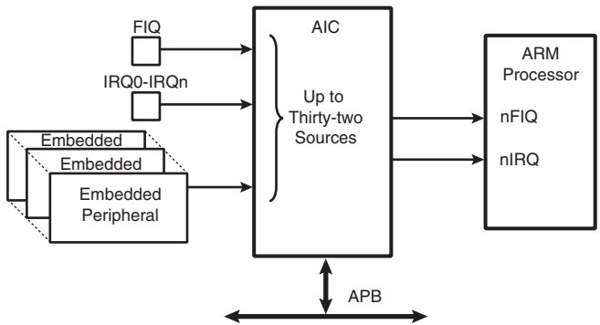
Figure 29-1. Block Diagram
