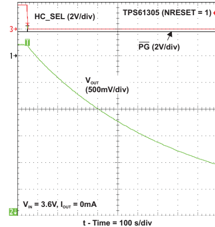
Figure 86. Shutdown (HC_SEL = 1)
