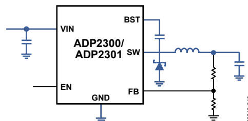
Figure 49. Typical Application Circuit with High Current Traces Shown in Blue
