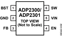
Figure 3. Pin Configuration
