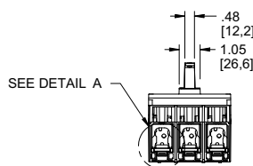
4896C-022-01 Top View Dimensions: Overall Width: 7.52 [191,0] Pin 1 to Pin 2: 6.22 [158,0] Pin 1 to Pin 3: 1.38 [35,0] Pin 1 to Pin 4: 1.30 [33,0] Pin 1 to Pin 5: 2.06 [52,4] Pin 1 to Pin 6: 1.38 [35,0] Pin 1 to Pin 7: 1.00 [25,5] Pin 1 to Pin 8: 1.76 [44,7] Pin 1 to Pin 9: 2.60 [66,1] Pin 1 to Pin 10: 5.57 [141,5] Pin 1 to Pin 11: 5.74 [145,8] Pin 1 to Pin 12: 6.52 [165,5] Pin 1 to Pin 13: 1.37 [34,8] Pin 1 to Pin 14: 4.12 [104,7] Pin 1 to Pin 15: 1.38 [35,0] Pin 1 to Pin 16: 0.20 [5,1] (MOUNTING HOLE) Side View Dimensions: Overall Height: 5.00 [127,0] Pin 1 to Pin 2: 3.44 [87,4] Pin 1 to Pin 3: 3.24 [82,4] Pin 1 to Pin 4: 2.87 [72,9] Pin 1 to Pin 5: 3.74 [95,1] Pin 1 to Pin 6: 4.25 [108,0] Pin 1 to Pin 7: 1.91 [48,5] Pin 1 to Pin 8: 19.9° OFF Pin 1 to Pin 9: 19.5° ON Pin 1 to Pin 10: 21.5° TRIPPED
