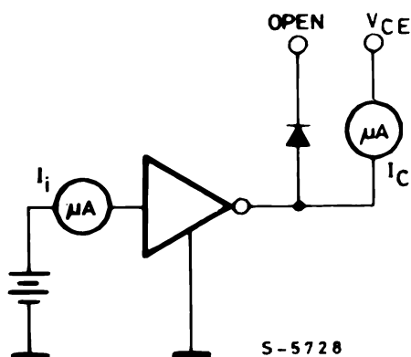
Figure 7. Input current (OFF)
