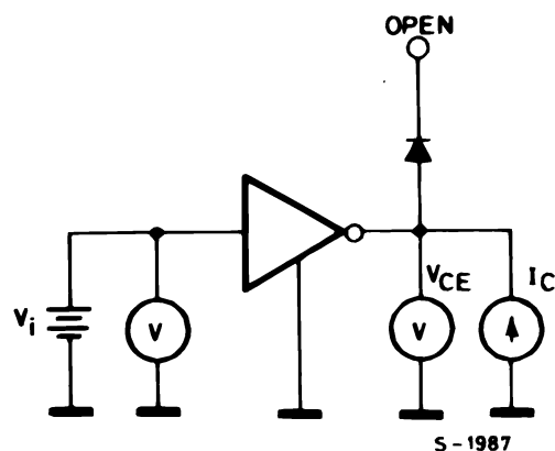
Figure 8. Input voltage
