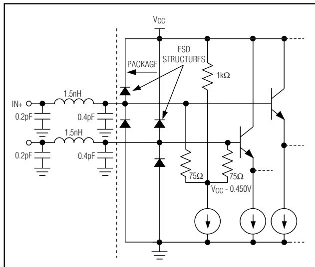
Figure 3. Input Structure
