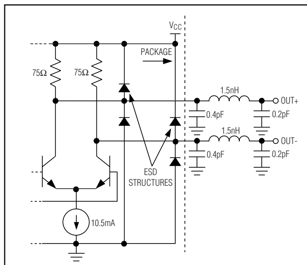
Figure 4. Output Structure
