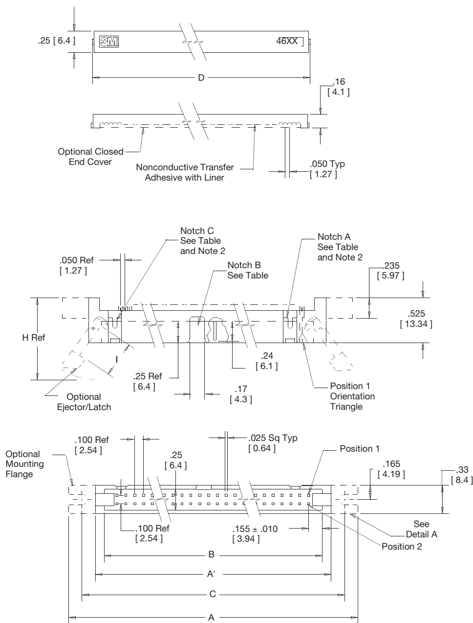
Slotted Mounting Flange 46XX-XXX0
