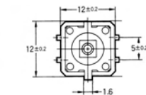
PCB Mounting (Top View) (Single-sided PCB, t=1.6 ) Two, 1.8 \pm 0.05 dia. (For positioning boss)
