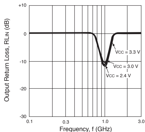
OUTPUT RETURN LOSS vs. FREQUENCY AND VOLTAGE
