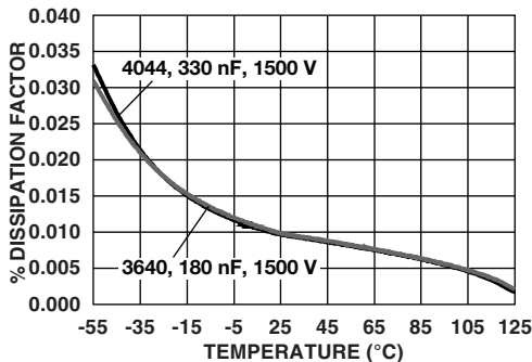
DISSIPATION FACTOR VS. TEMPERATURE
