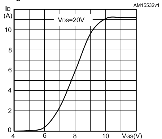
Figure 7: Transfer characteristics
