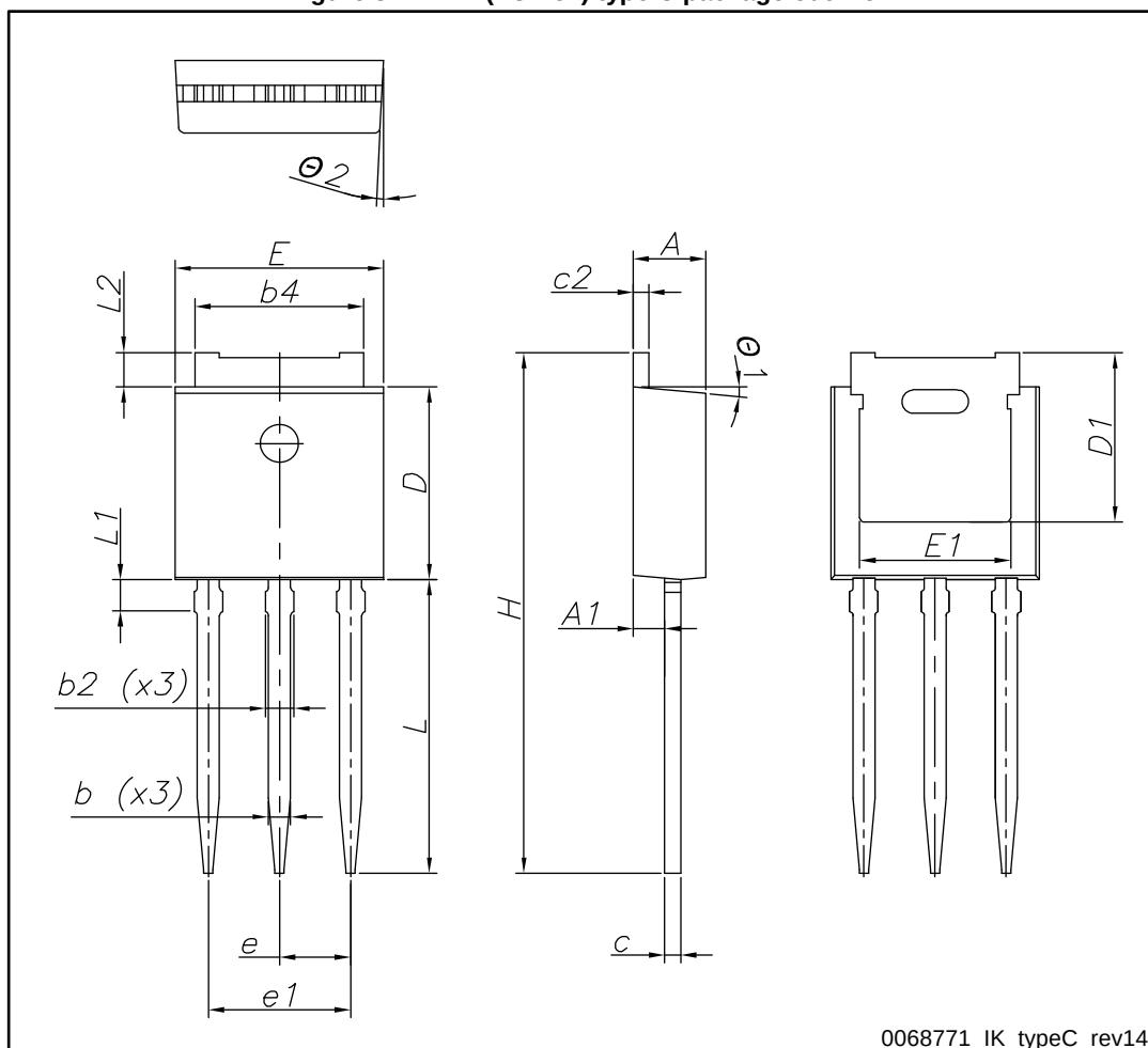
Figure 31: IPAK (TO-251) type C package outline
