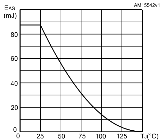
Figure 14: Maximum avalanche energy vs starting T_J
