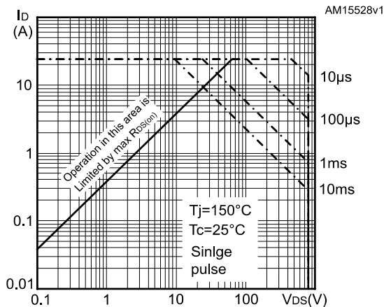
Figure 2: Safe operating area for DPAK and IPAK
