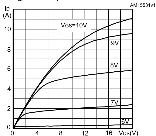
Figure 6: Output characteristics
