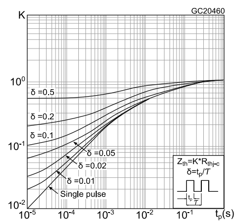
Figure 3: Thermal impedance for DPAK and IPAK
