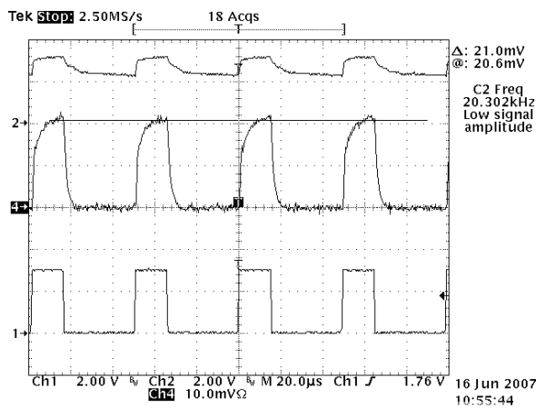
PWM Minimum on time 15μs 20kHz CH1: PWM Signal CH2: Anode of LED CH4: LED current 10mA/div
