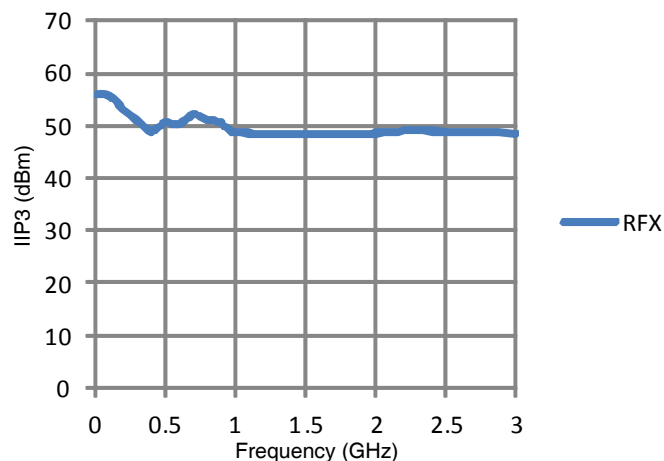
Figure 15. Input IIP3 RFC-RFX
