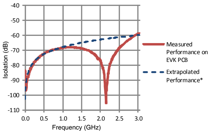
Figure 14. RFX-RFC Isolation
