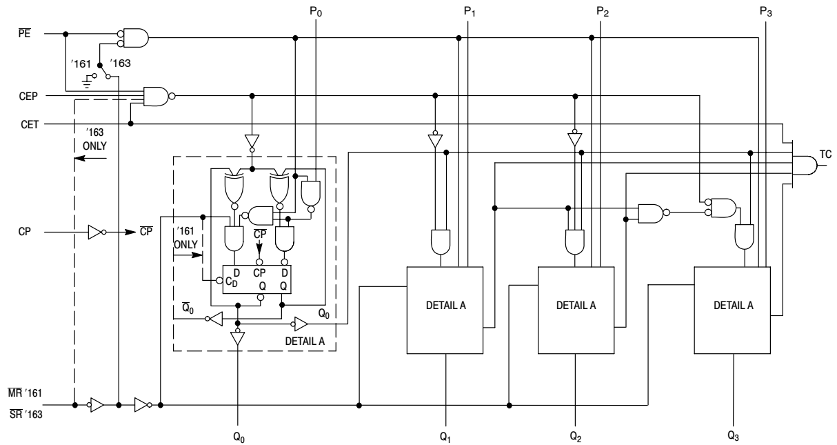
Figure 4. Logic Diagram
