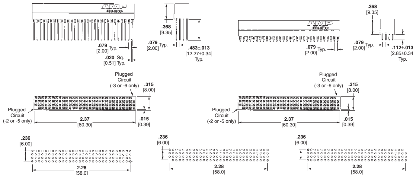
Recommended PC Board Layout for 1375799-1, 1375799-4, 1375800-1, 1375800-4
