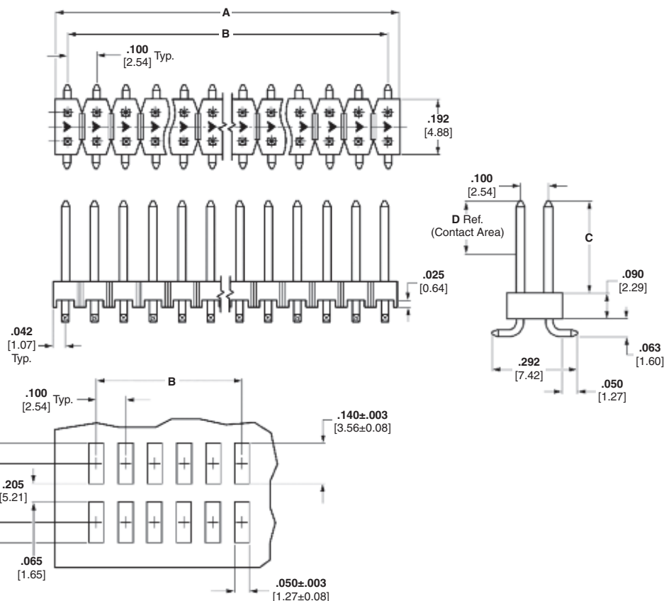
Recommended Etched Circuit Layout (Using .008 [0.20] thick stencil)
