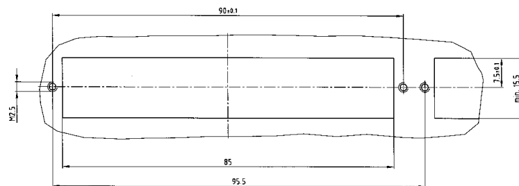
Panel cutout
