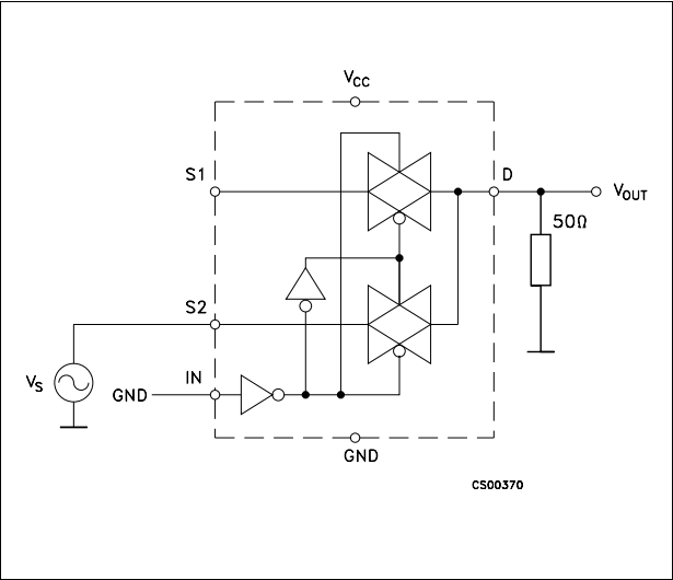
Figure 6. Channel-to-channel crosstalk
