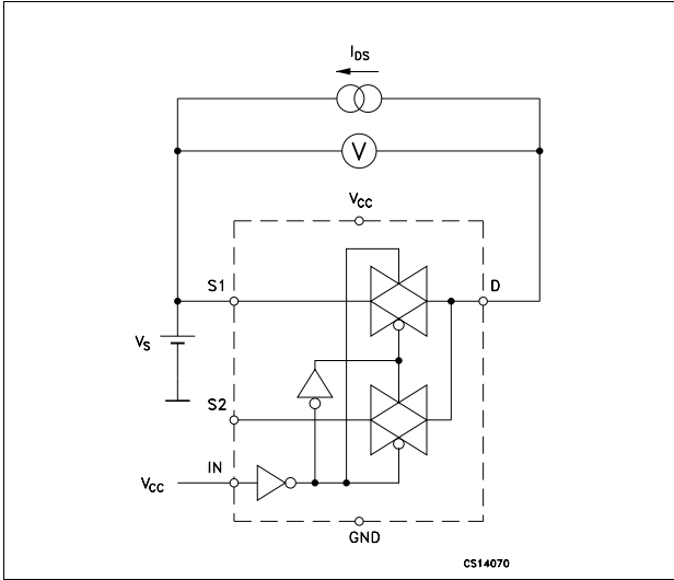
Figure 5. OFF leakage
