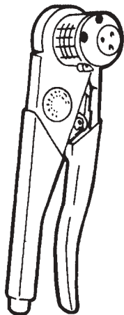
8365 with locator 8365-02
