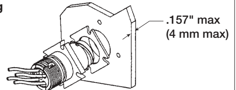
Rear Mounting
