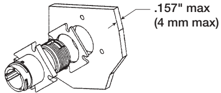
Front Mounting
