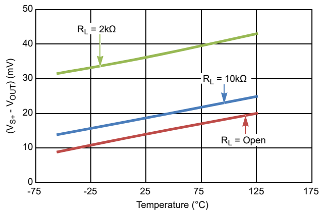
Figure 22. ( V_S = \pm 1.5V ) V_{OH} vs Temperature
