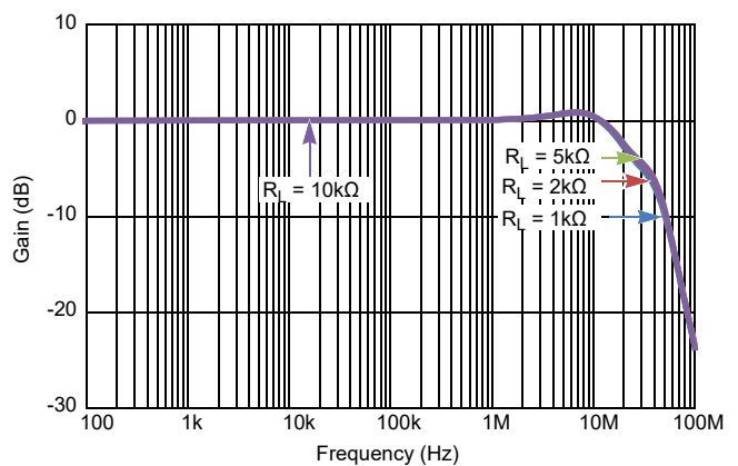
Figure 41. Frequency Response vs Load Resistance
