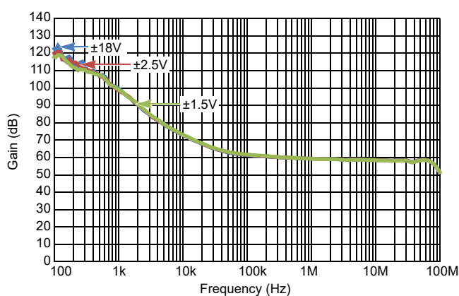
Figure 44. Crosstalk Rejection
