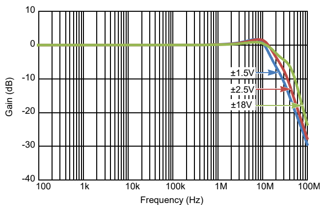
Figure 43. Frequency Response vs Supply Voltage
