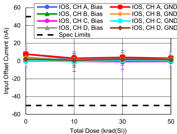
Figure 61. Input Offset Current vs TID ( V_S = \pm 18V )
