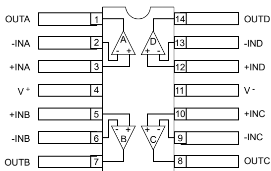
Figure 3. Pin Assignments - Top View
