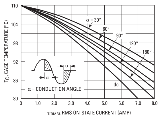
Figure 1. Current Derating
