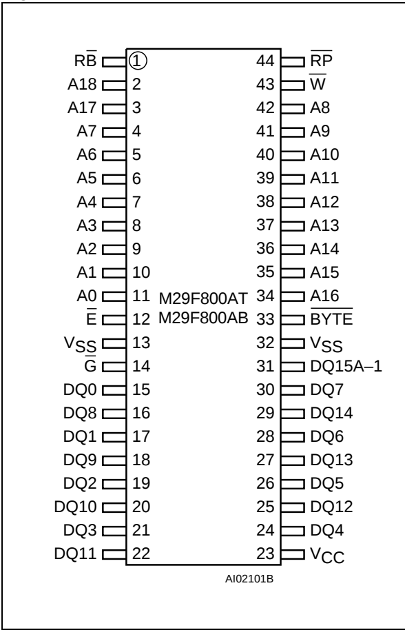
Figure 3. SO Connections
