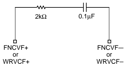
Figure 4. Recommended Loop Filter Values
