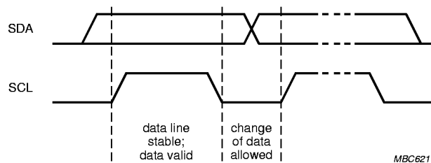
Fig.11 Bit transfer.
