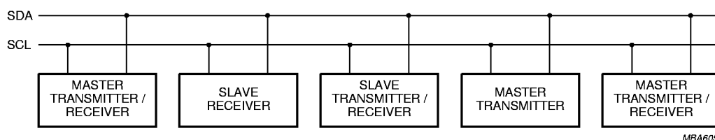
Fig.13 System configuration.
