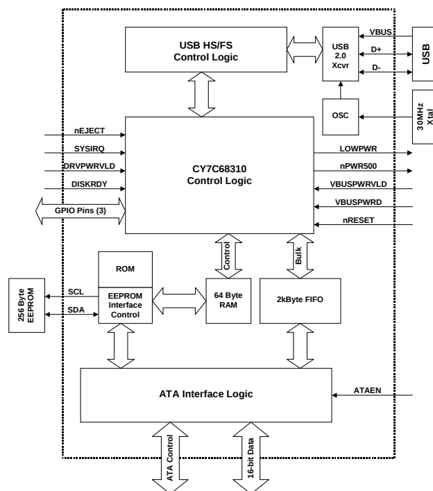
Figure 1-1. Block Diagram
