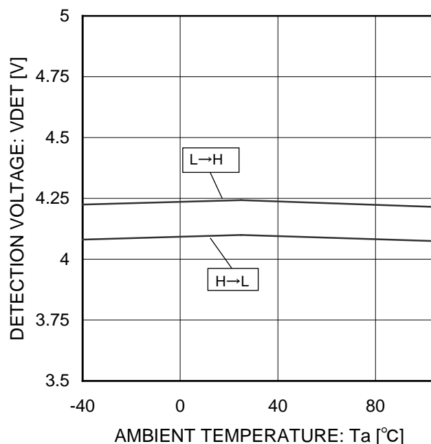
Figure 10. Detection Voltage vs Temperature
