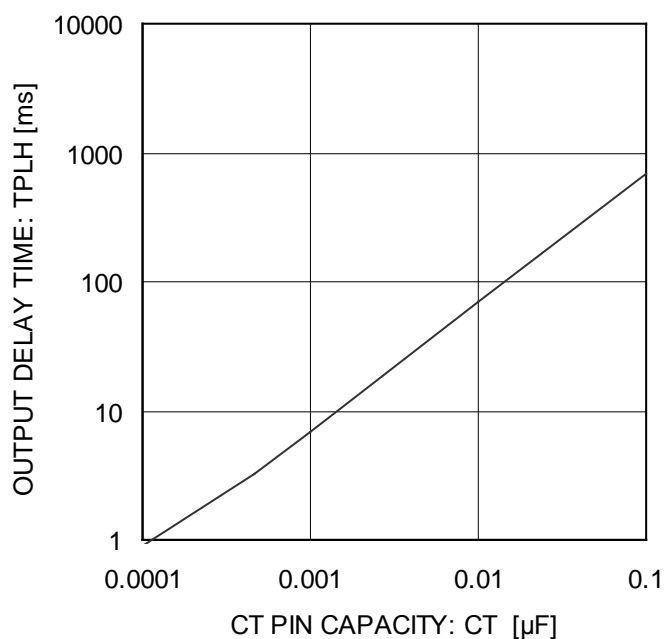
Figure 8. T RESET Transmission Delay Time vs Capacitance
