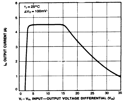
Figure 3. Current Limit
