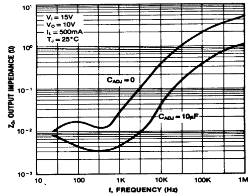
Figure 11. Output Impedan
