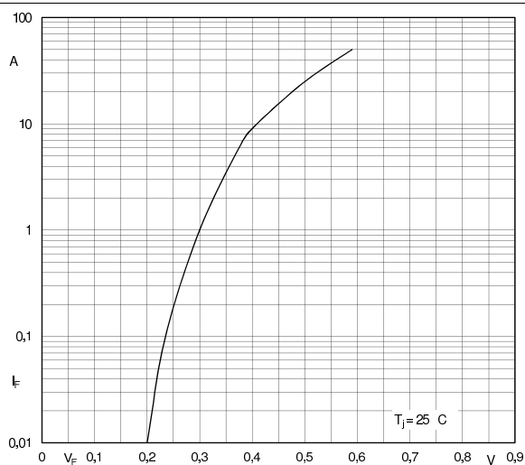
Fig.1: Forward characteristics (typical value)
