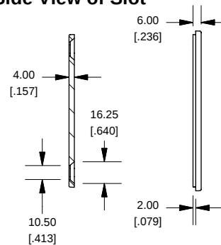
SECTION C-C Side View of Slot
