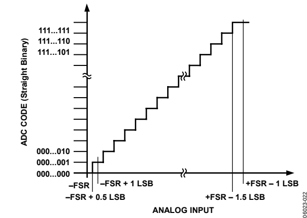
Figure 23. ADC Ideal Transfer Function
