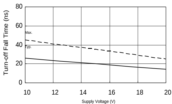
Figure 10B. Turn-off Fall Time vs. Supply Voltage
