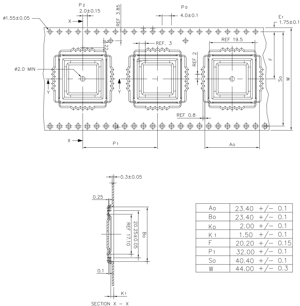
Figure A-3. 144-Pin LQFP PGE Package Carrier Tape
