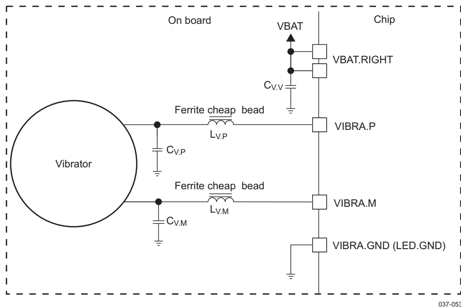
Figure 6-3. Vibrator H-Bridge
