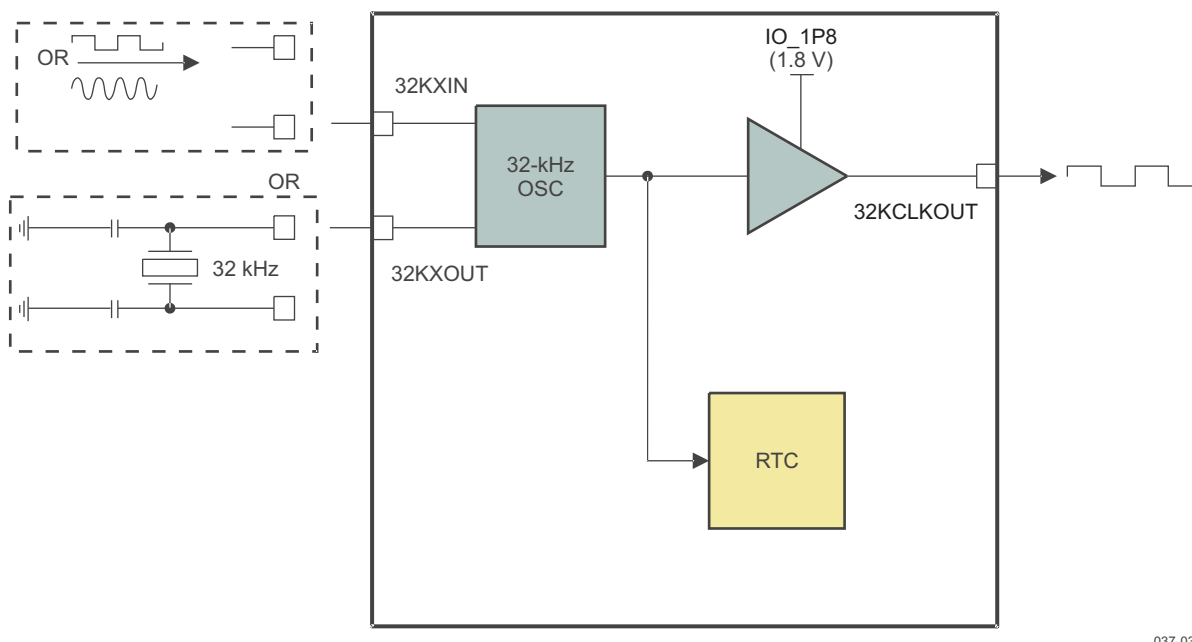
Figure 11-11. 32.768-kHz Clock Output Block Diagram
