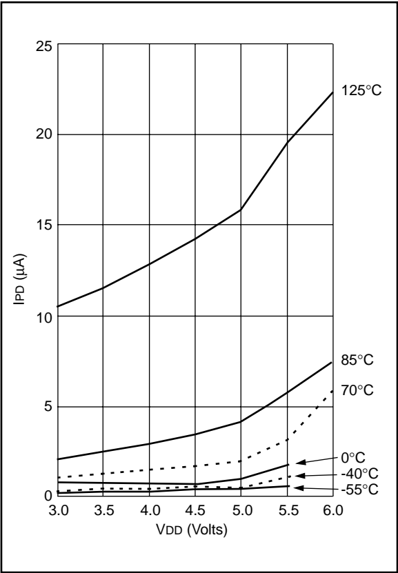
FIGURE 17-7: MAXIMUM I PD VS. V DD WATCHDOG DISABLED
