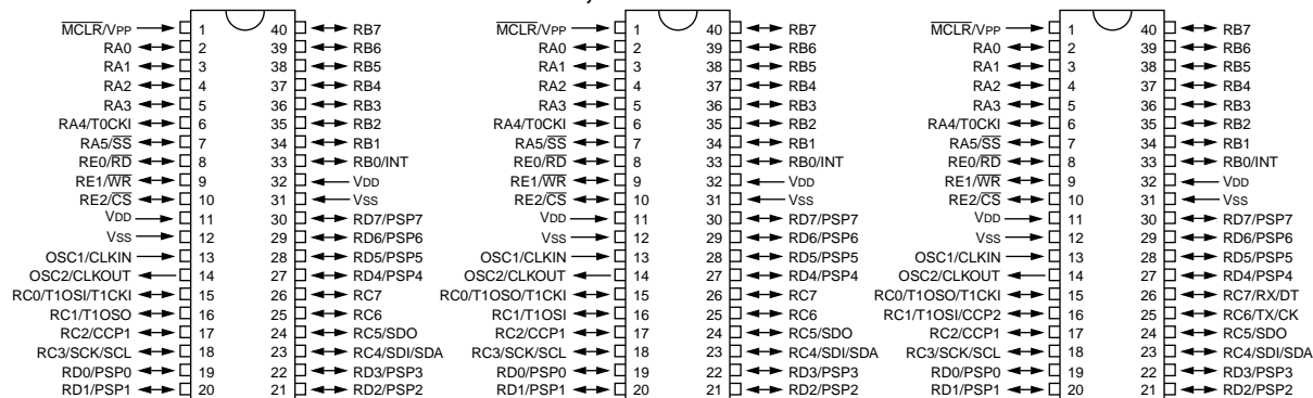
PIC16C64
