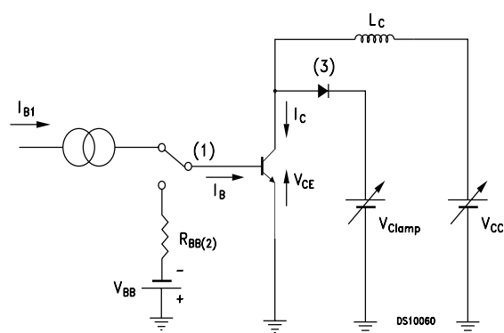
Figure 10. Reverse biased safe operating area
