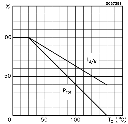
Figure 2. Derating curve
