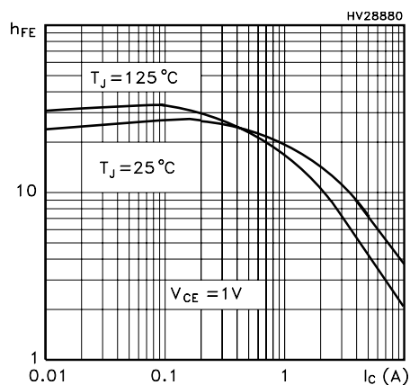
Figure 5. DC current gain at V_{CE} = 1 V
