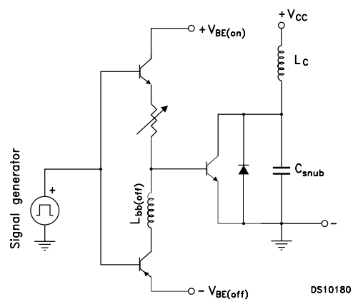
Figure 9. Power losses and inductive load switching
