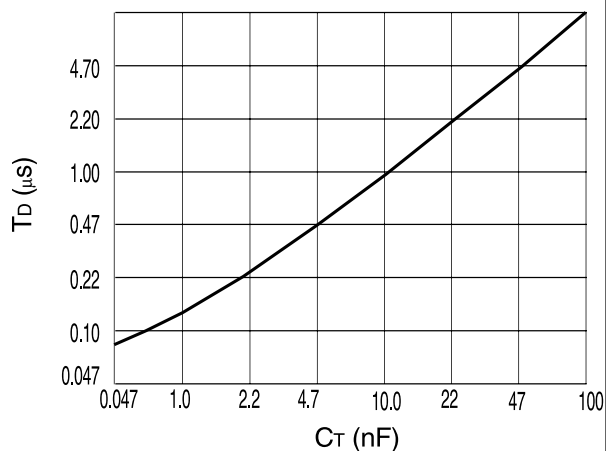
Deadtime vs C_T (3k R_T 100k)
