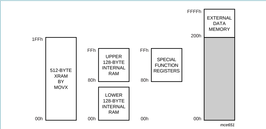
Fig 9. Internal and external data memory address space with EXTRAM = 0
