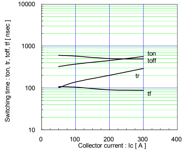
Switching time vs. Collector current (typ.) Vcc=600V, VGE=±15V, RG=3.0Ω, Tj=125°C
