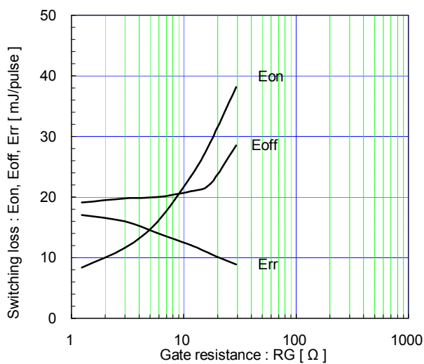
Switching loss vs. Gate resistance (typ.) Vcc=600V, Ic=200A, VGE=±15V, Tj=125°C
