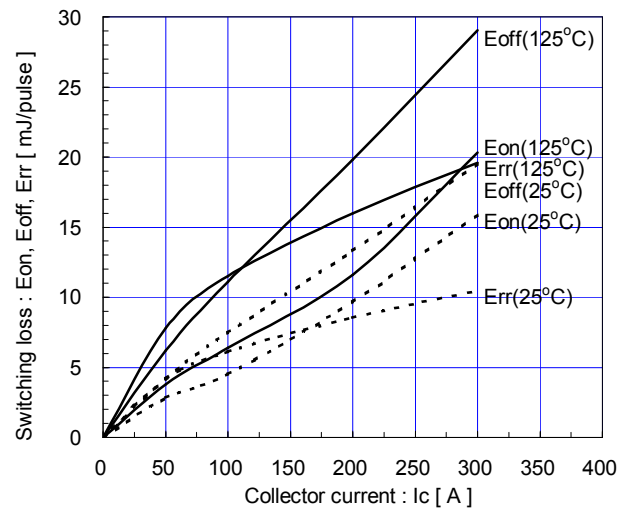
Switching loss vs. Collector current (typ.) Vcc=600V, VGE=±15V, RG=3.0Ω
