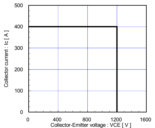
Reverse bias safe operating area (max.) +VGE=15V, -VGE ≤ 15V, RG ≥ 3.0Ω, Tj ≤ 125°C
