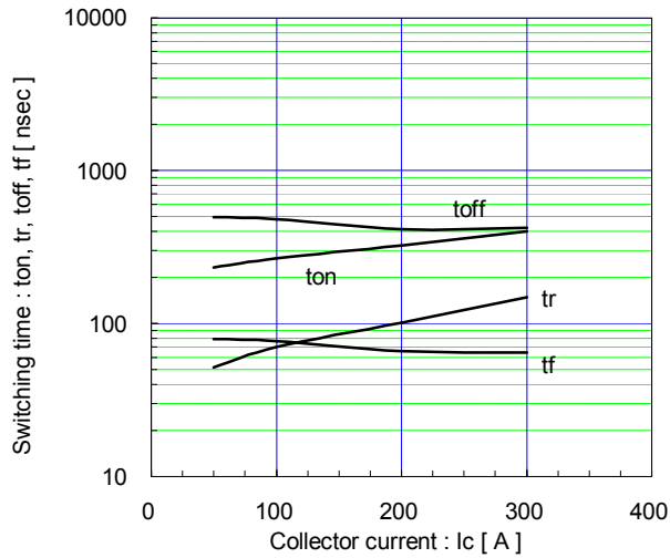
Switching time vs. Collector current (typ.) Vcc=600V, VGE=±15V, RG=3.0Ω, Tj=25°C
