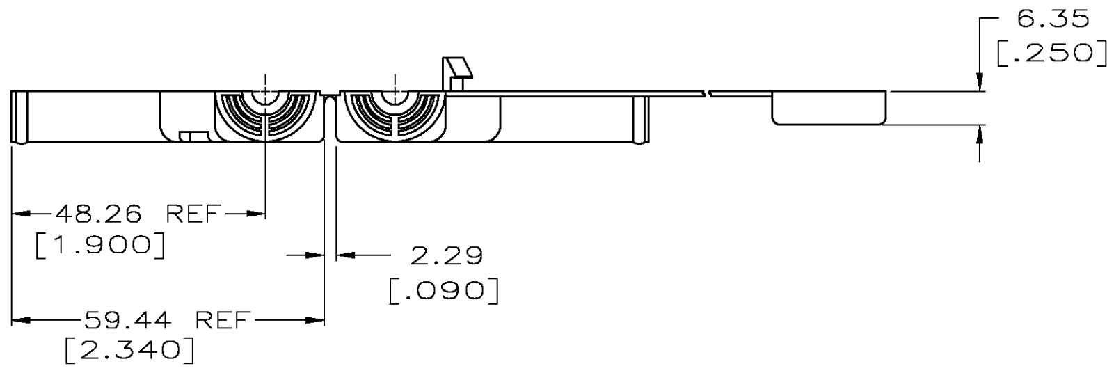
VIEW B
