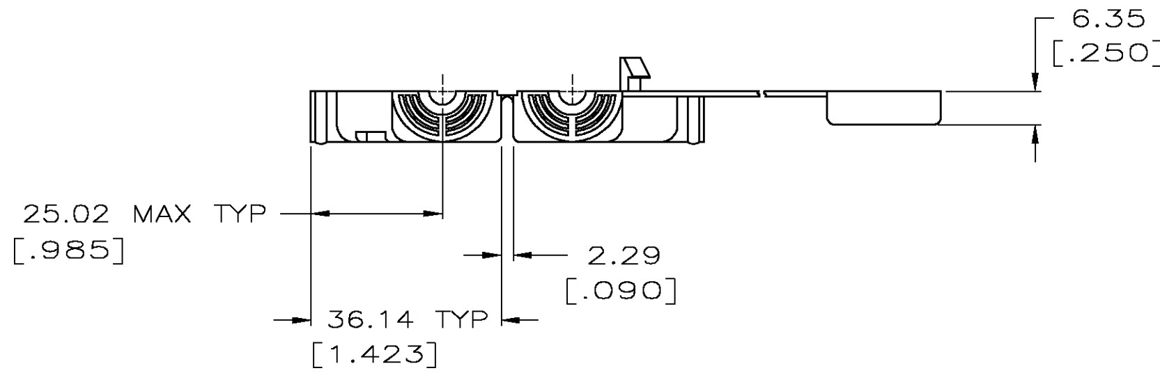
VIEW A
