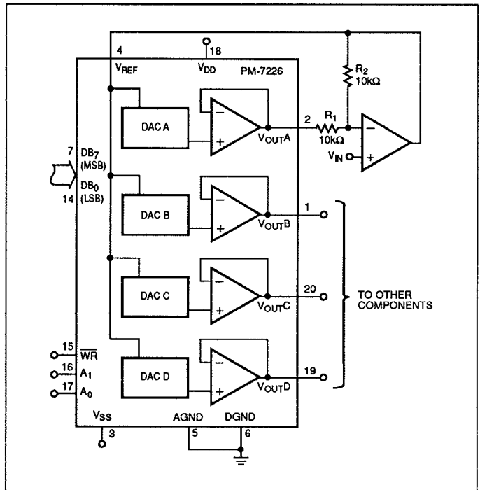
FIGURE 22: Programmable DAC Reference
