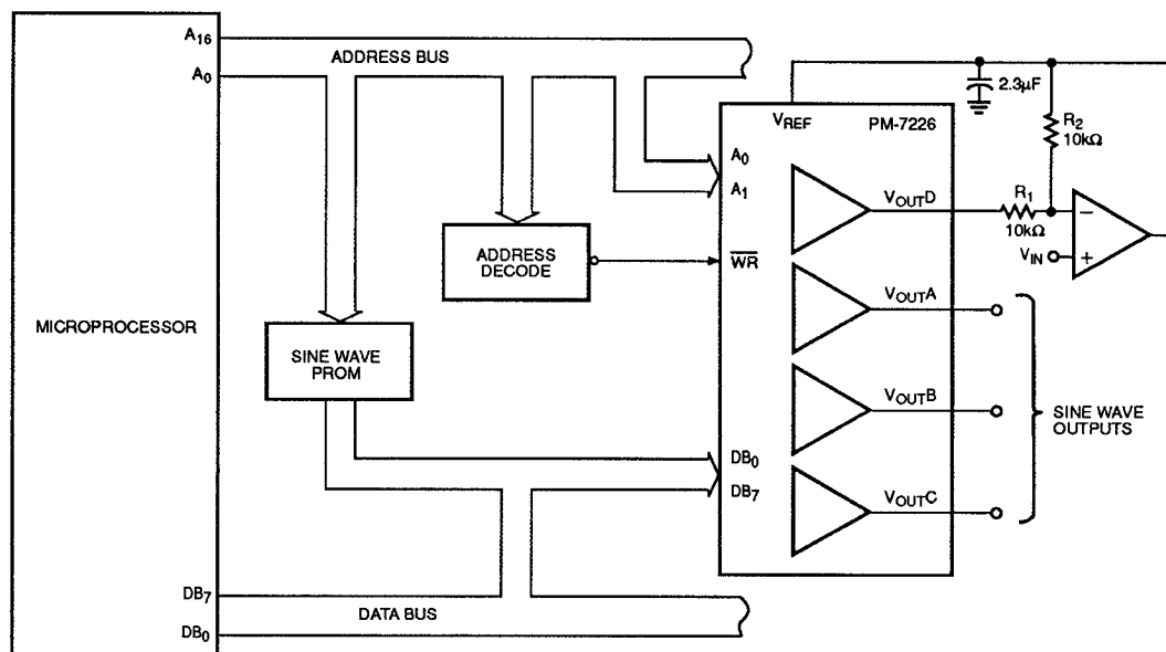
FIGURE 24: 3-Phase Sine Wave Generator Circuit (Under Microprocessor Control)
