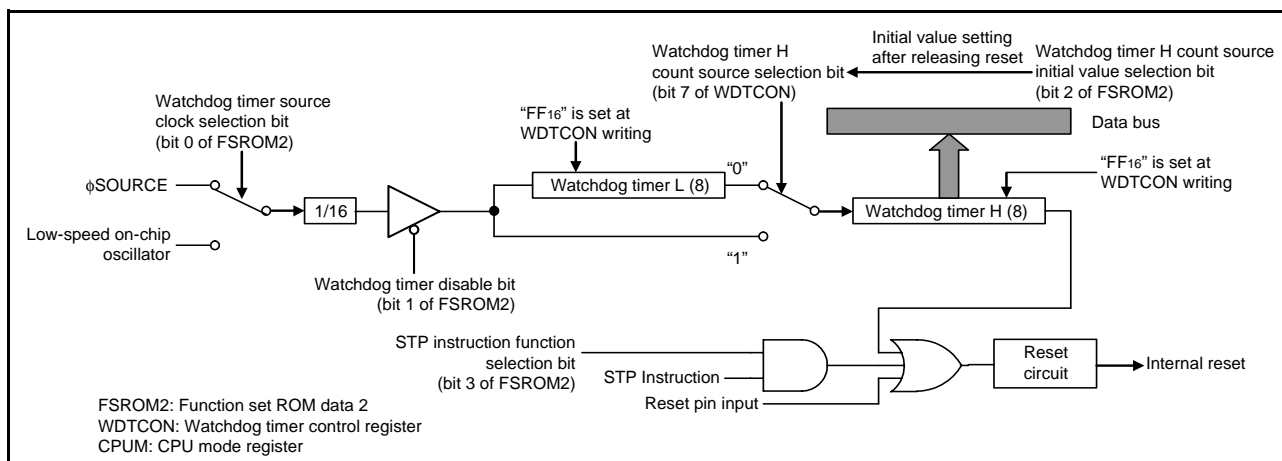
Fig 56. Block diagram of watchdog timer
