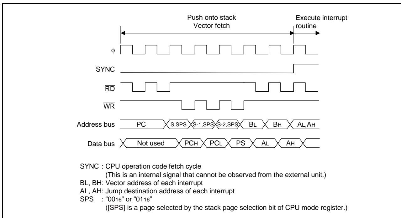
Fig 22. Interrupt sequence
