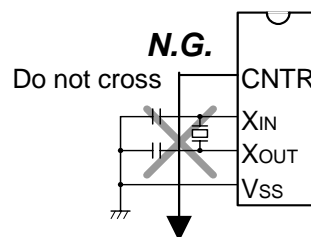
Fig 78. Wiring for a large current signal line/Writing of signal lines where potential levels change frequently
