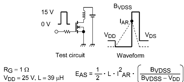
Fig. 8.15 Test Circuit/Waveform
