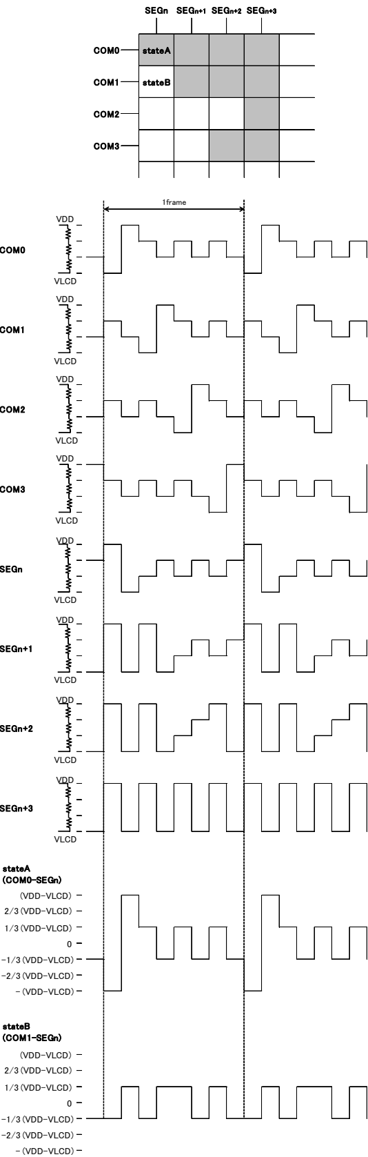
Figure 16. LCD waveform at line inversion (1/3bias)
