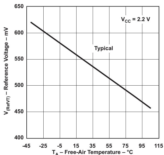
Figure 15. V (RefVT) vs Temperature, V CC = 2.2 V
