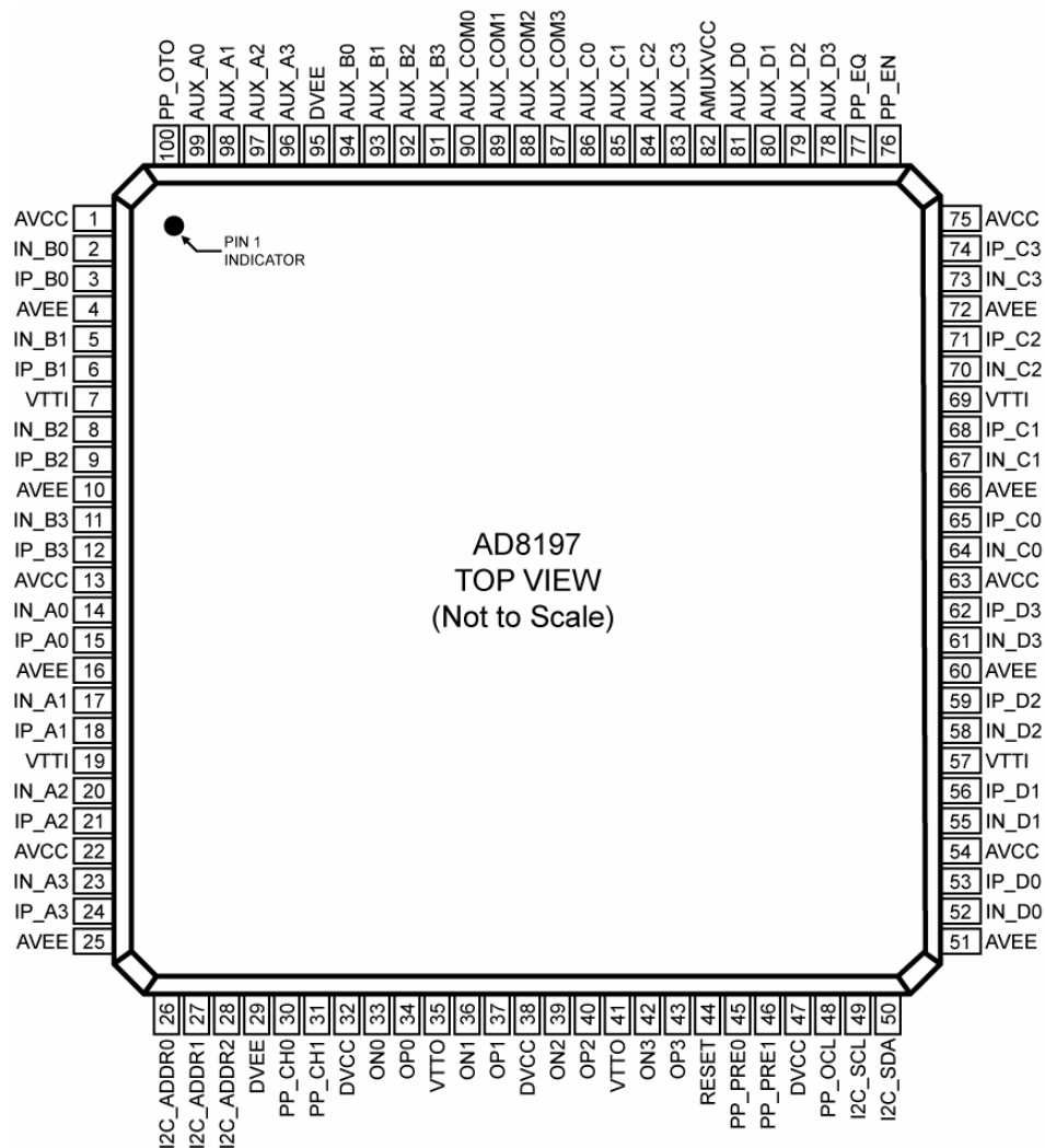
Figure 3. Pin Configuration
