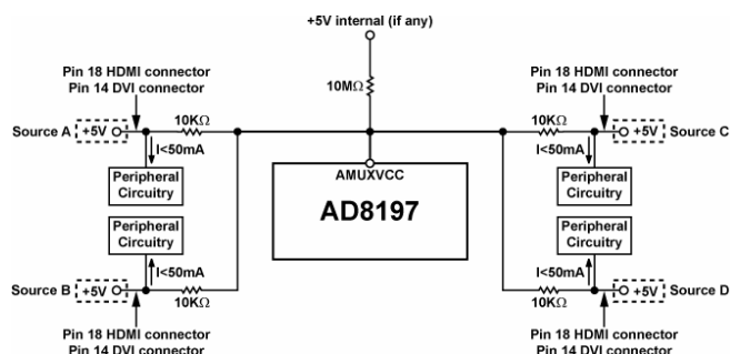
Figure 28. Suggested AMUXVCC Power Scheme
