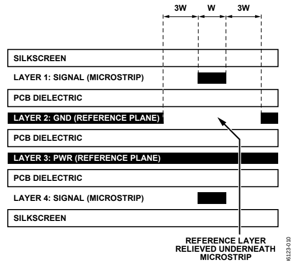
Figure 33. Example Board Stackup
