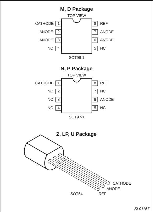
Figure 1. Pin Configuration
