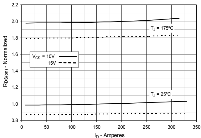
Fig. 5. R_{DS(on)} Normalized to I_D = 150\text{A} Value vs. Drain Current
